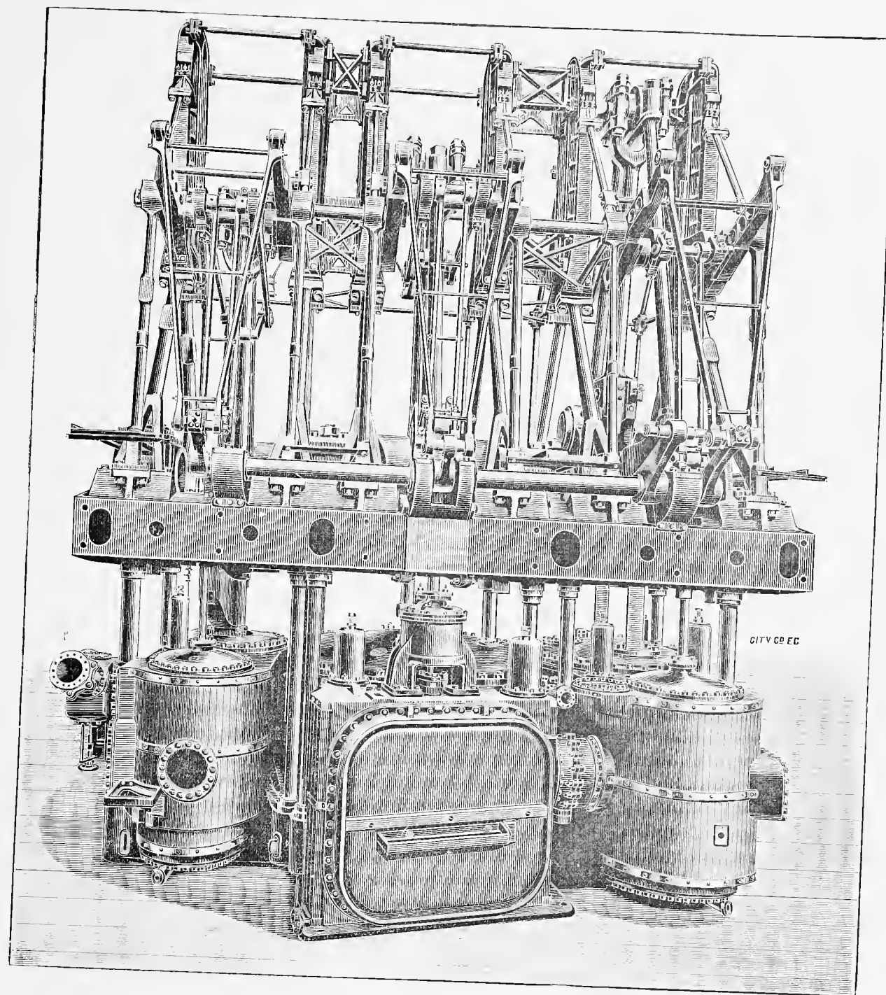
TRIPLE-EXPANSION STEEPLE ENGINES OF THE STEAMER BANSHEE.—Built by Laird Bros.
